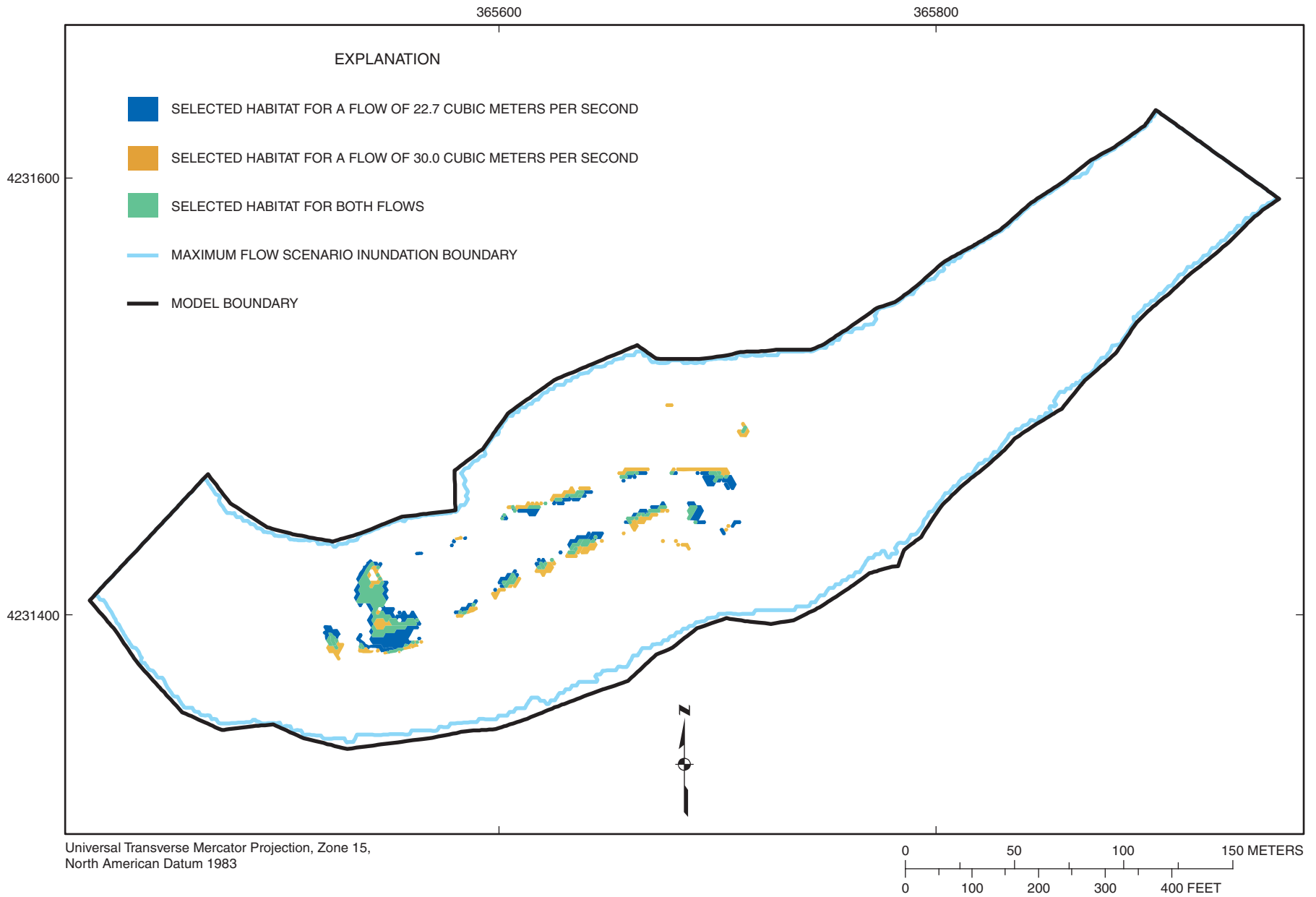
Figure 4-63. Selected habitat area distribution for habitat categories 16, 17 combined (channel catfish) at flows of 22.7 and 30.0 cubic meters per second at Marais des Cygnes River site MDC2.
